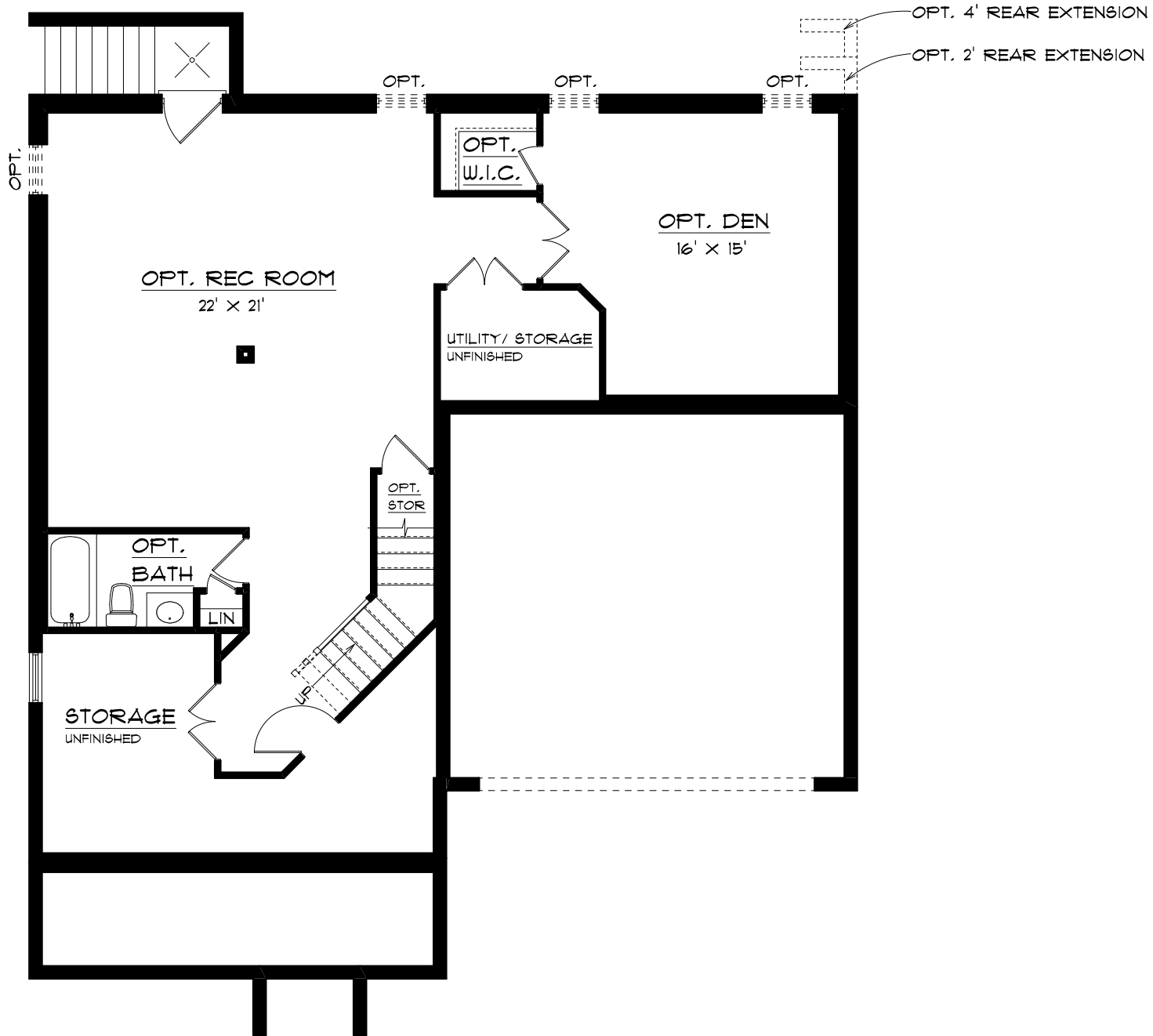
OPT. FINISHED BASEMENT PLAN
